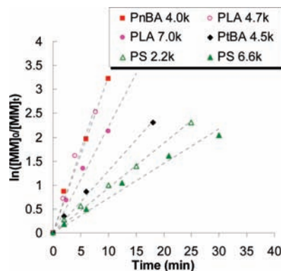
Figure 2. Dependence of \ln([MM]_0/[MM]_t) on time for ROMP of MMs. Conditions: [MM] 0 = 0.05 M in THF at room temperature, [MM/C] 0 = 200. The dashed lines are best-fit lines.
